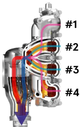
4-2-1 Performance Tuned Exhaust
