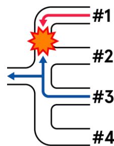
Exhaust interference in regular 4-1 exhaust manifold
